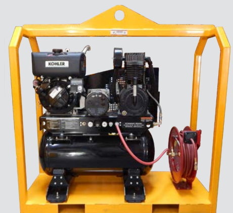
Summit Compressor/Generator Powered by a diesel/gas engine (30 gallon, 80 gallon, 120 gallon or per customer specifications).
